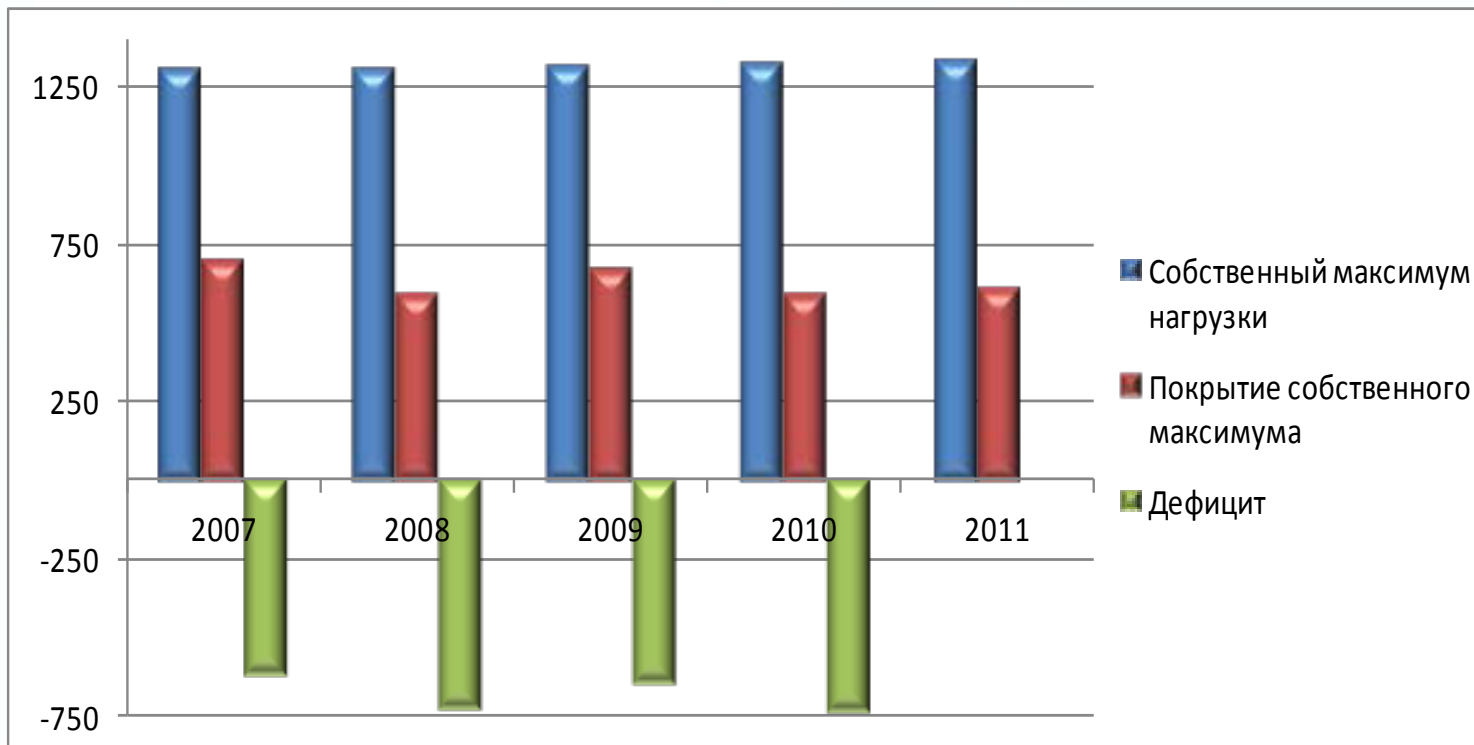
Power balance of Karelian energy system in 2007 - 2011
